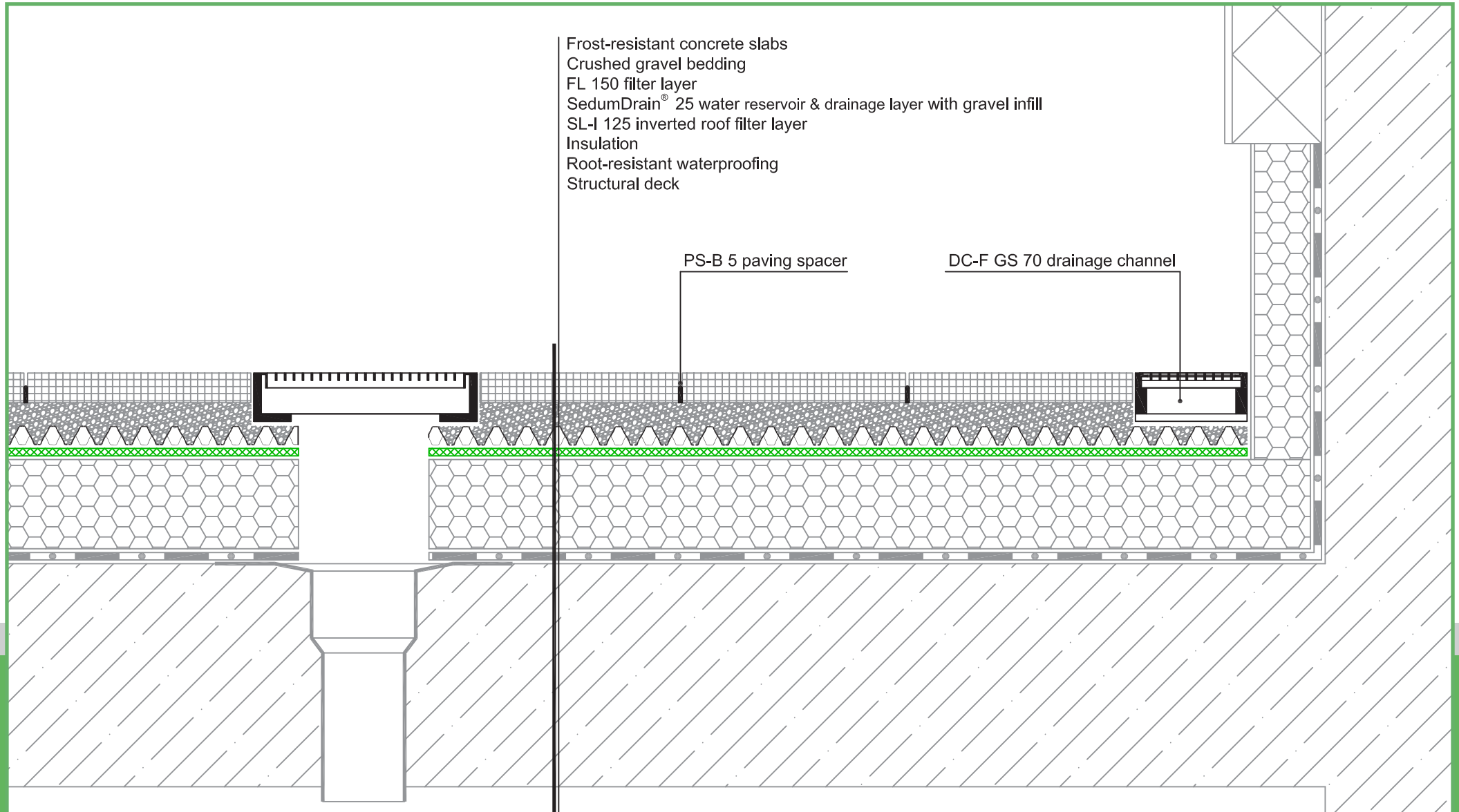
Wall connection DC-F fixed height drainage channel
