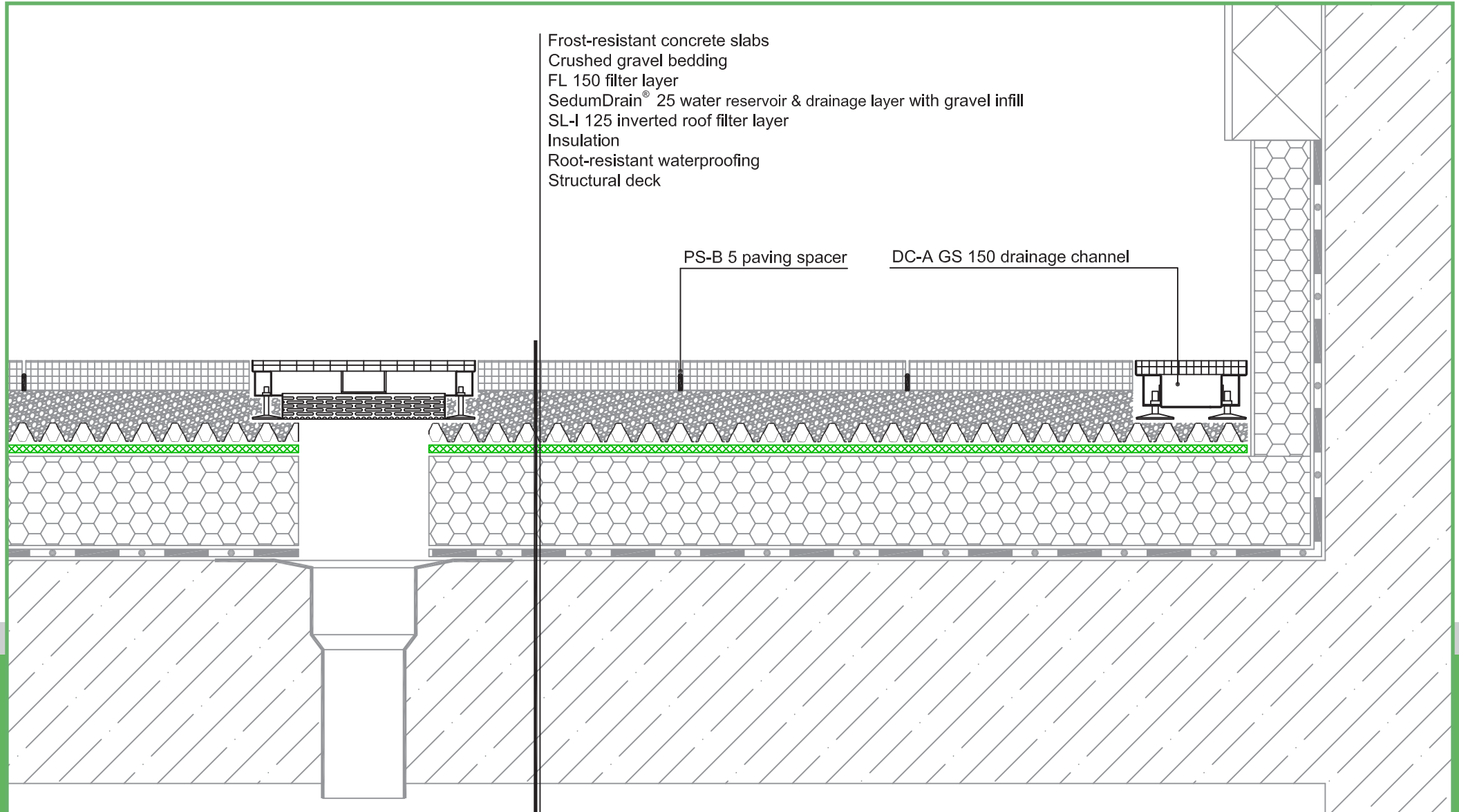
Wall connection DC-A adjustable height drainage channel
