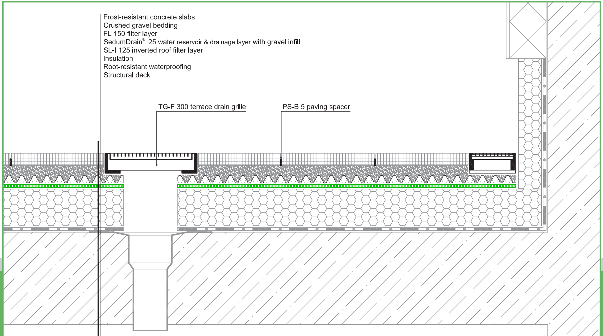
Roof terrace with outlet TG-F fixed height terrace grille
