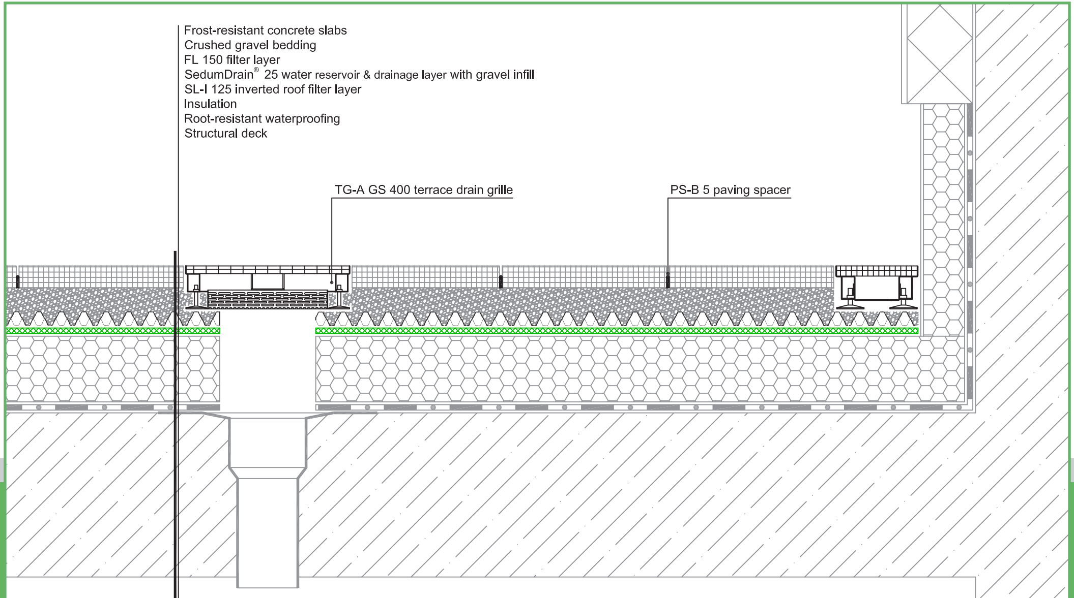
Roof terrace with outlet TG-A adjustable height terrace grille
