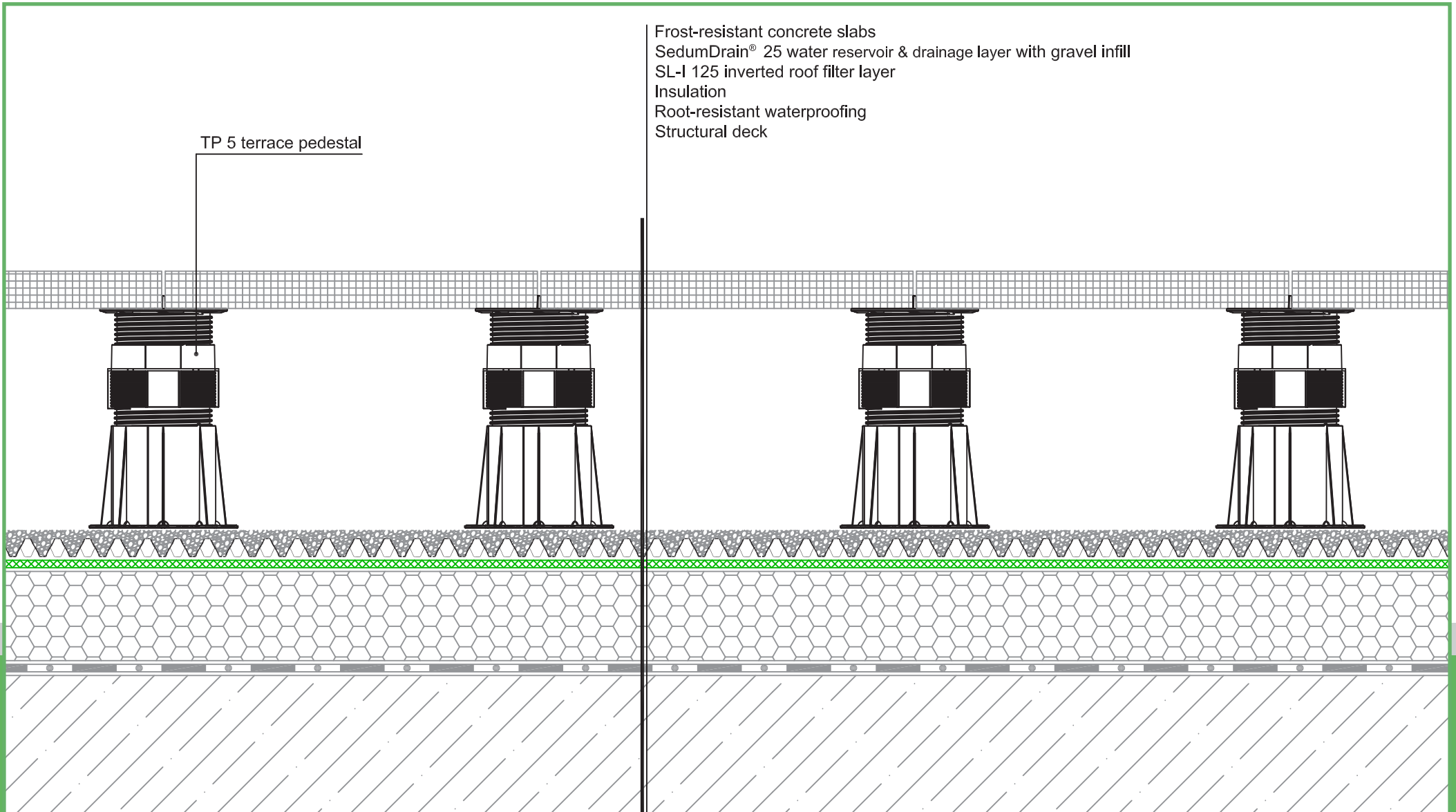
Raised floor roof terrace TP terrace pedestal
