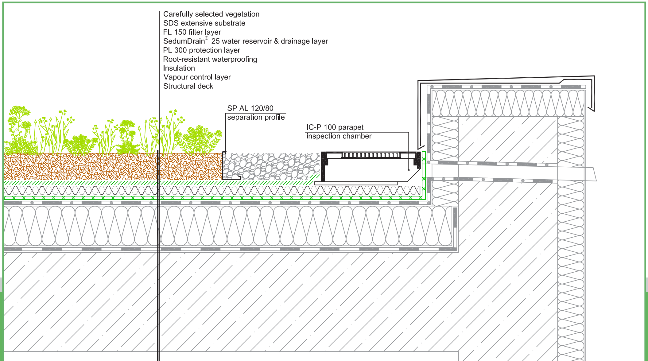
Parapet with water spout IC-P parapet inspection chamber
