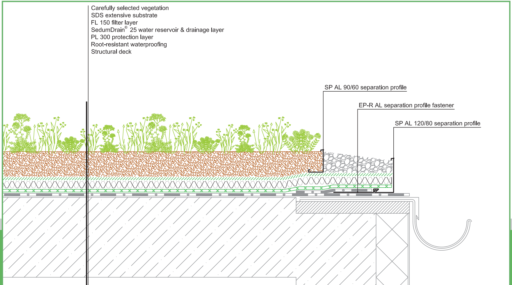
Gutter without parapet wall EP-R separation profile fastener
