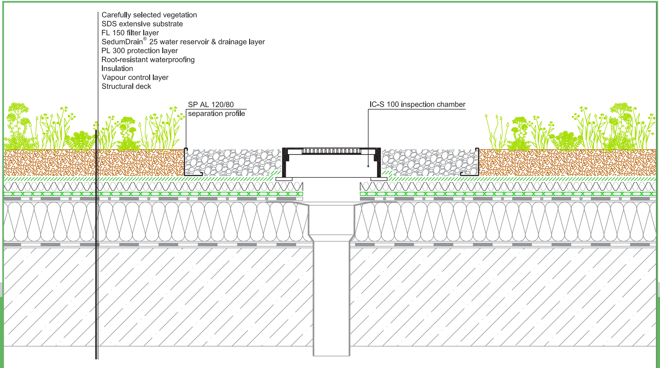
Extensive green roof outlet IC-S inspection chamber
